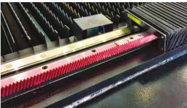
Linear axis with double pinion and rack drive.
