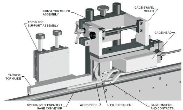
Fixed-size "rolling V" with auxiliary carbide top guide for a mix of long and short parts on TFD-24
