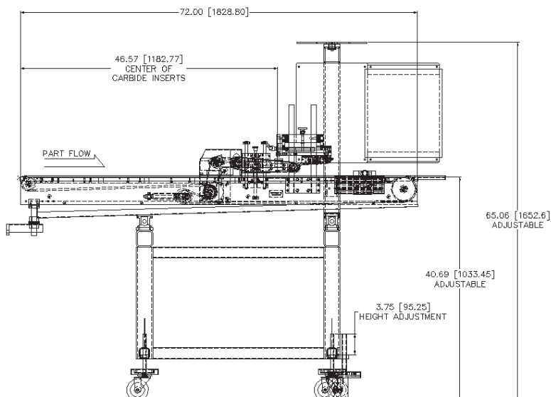
Fixed-size "rolling V" with auxiliary carbide top guide for a mix of long and short parts on TFD-24
