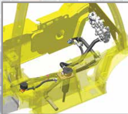
Hydraulic System
