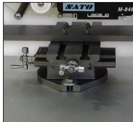
An XY adjustable head mounting allows for a wide range of adjustment for product changeovers.
