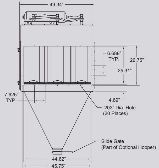
Inlet End View
