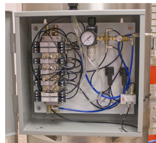
APS panel for 4 cartridges. Electric timers are available (non explosion proof)
