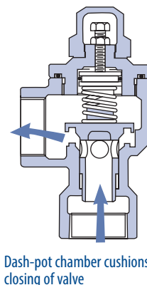
FIGURE 5. Bypass valve operation
